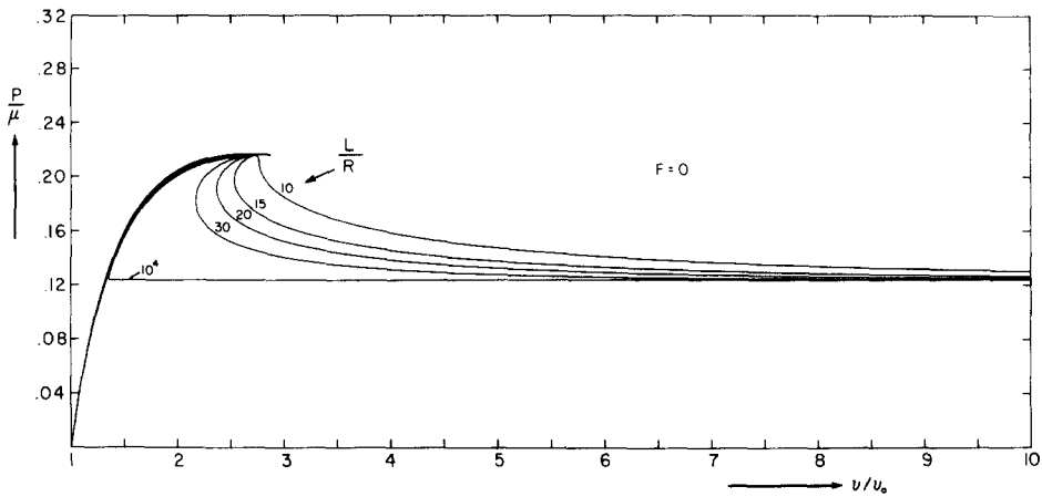
Fig. 15. Pressure-volume responses for tubes of different lengths.
